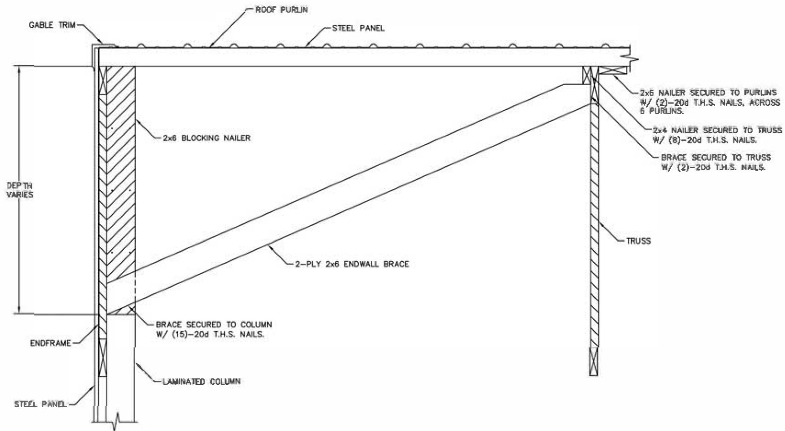
ENDWALL BRACE DETAIL
